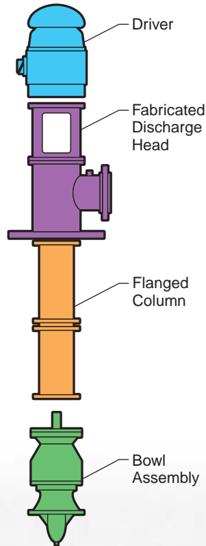
Model MVT-FF
